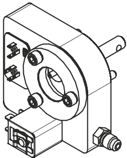
Fig.1. General view
