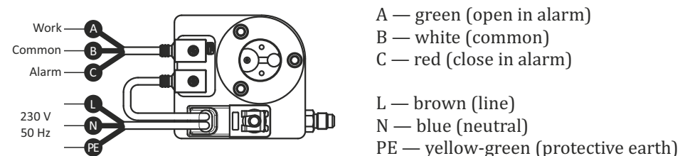
Fig.3. Electrical Connection
