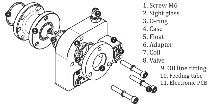
Fig.2. Assembly drawing
